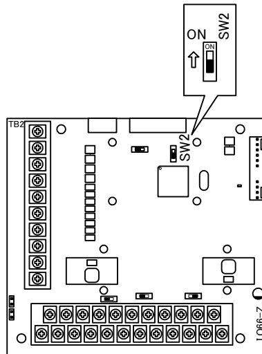
図6.1 PG信号入力切換
